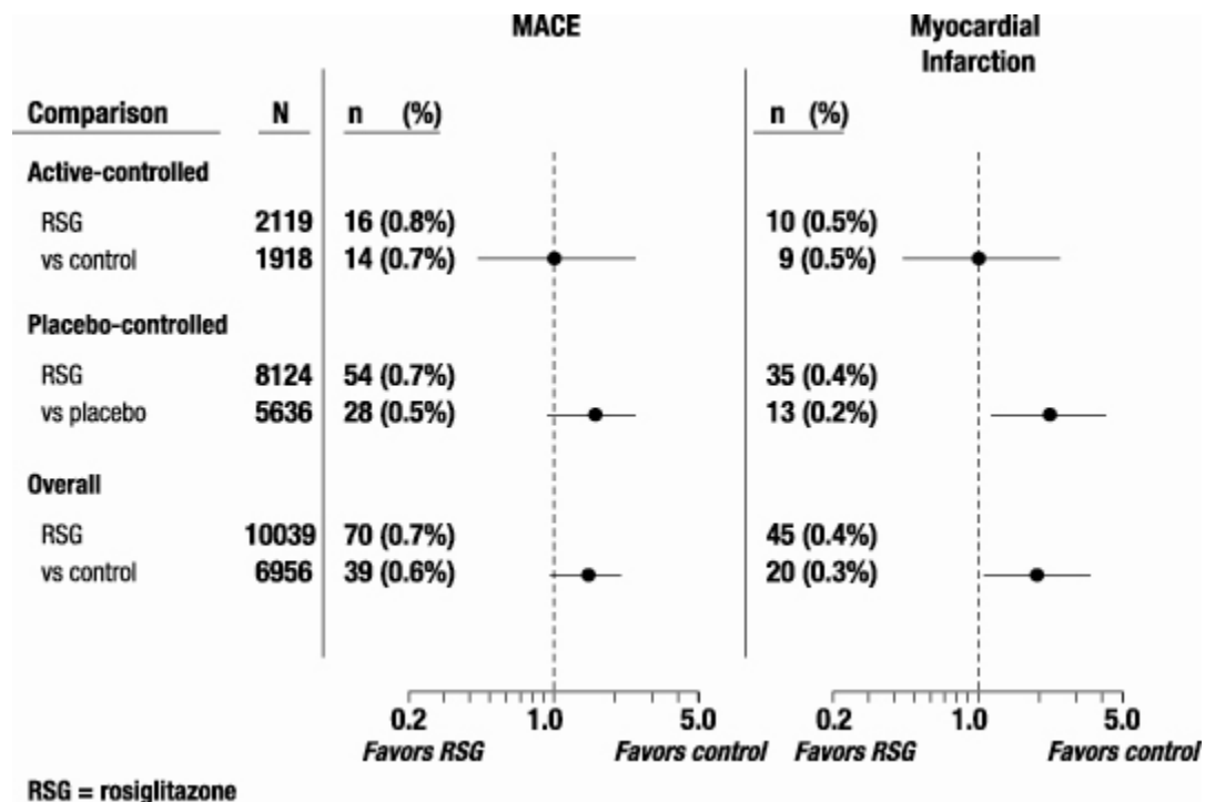
Figure 1. Forest Plot of Odds Ratios (95% Confidence Intervals) for MACE and Myocardial Infarction in the Meta-Analysis of 52 Clinical Trials
